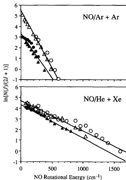
Fig. 2. Boltzmann plots of the NO( {}^2\Pi_{\Omega} ) rotational distributions obtained in the inelastic scattering of jet-cooled NO. The temperatures given in Table 1 are obtained from the slopes of the shown straight lines through the data.
