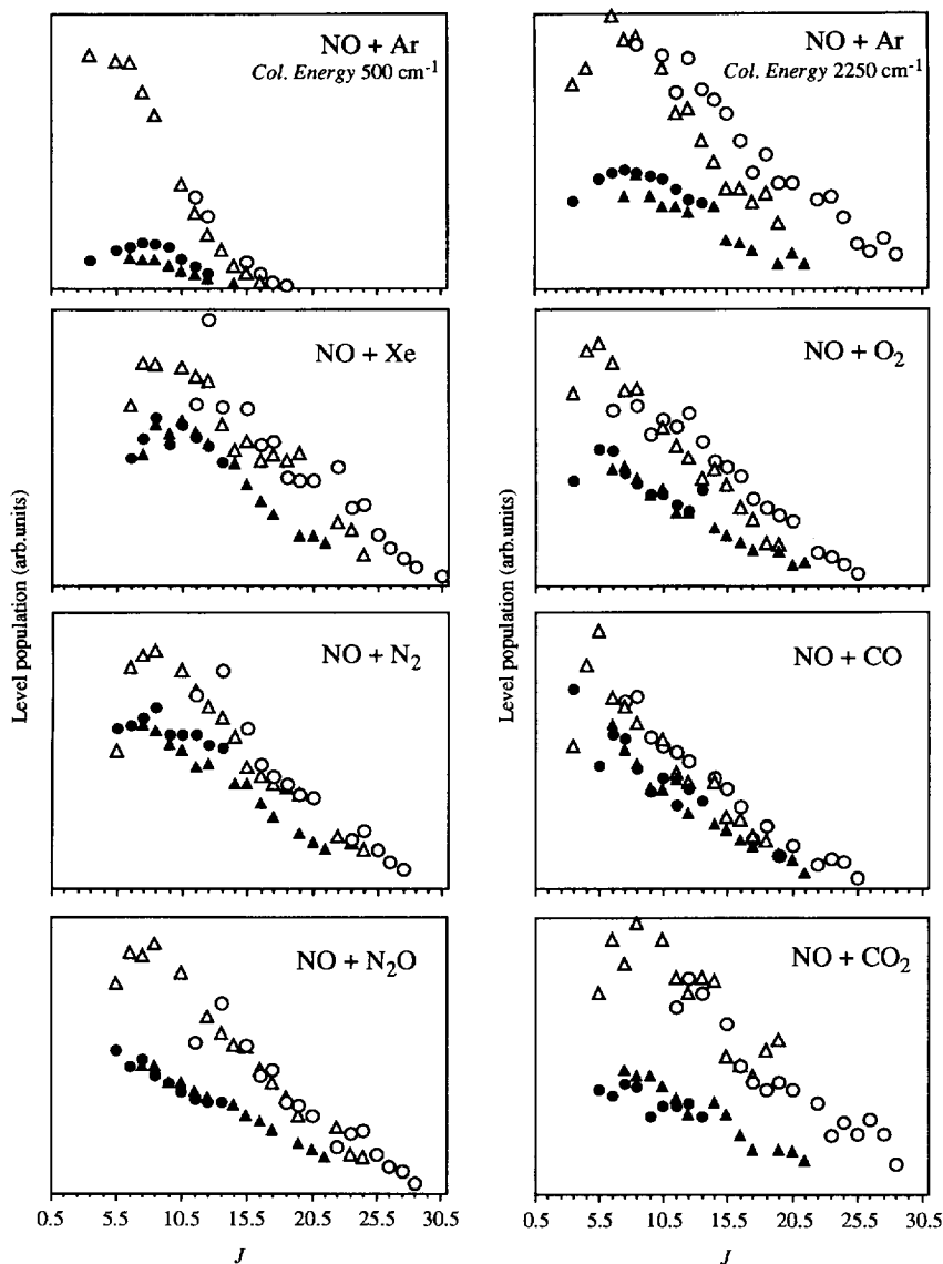
Fig. 1. NO( {}^2\Pi_{1/2} and {}^2\Pi_{3/2} ) rotational level distributions obtained in the inelastic scattering of jet-cooled NO at collisional energies listed in Table 1. Scattering of NO by Ar is carried out at two different collisional energies obtained by seeding NO in He or Ar. The populations of the \Pi(A'') and \Pi(A') A -doublet components are obtained from the Q and P/R branch lines of the NO ( A \leftarrow X ) transition, respectively. ( \Delta ) R_{11} + Q_{21} , ( \circ ) Q_{11} + P_{21} , ( \blacktriangle ) P_{22} + Q_{12} , ( \bullet ) Q_{22} + R_{12} .
